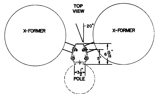
Typical Installation
